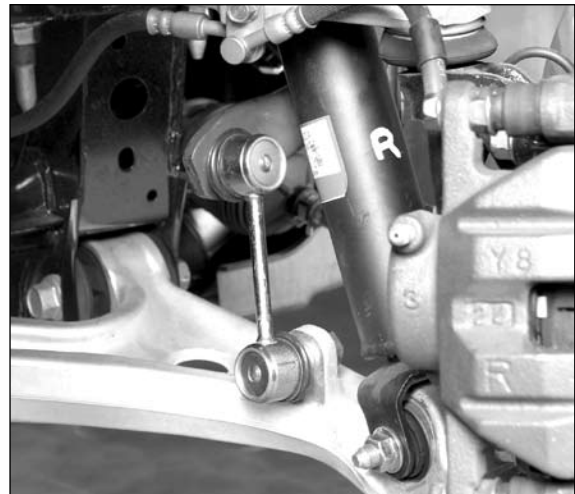
End link orientation.
